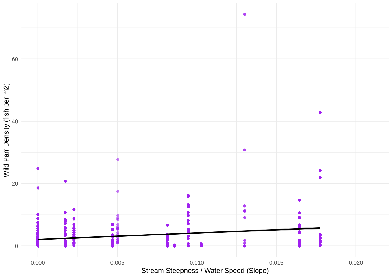
Effect of Waterflow Speed on Wild Precocious Parr Density
